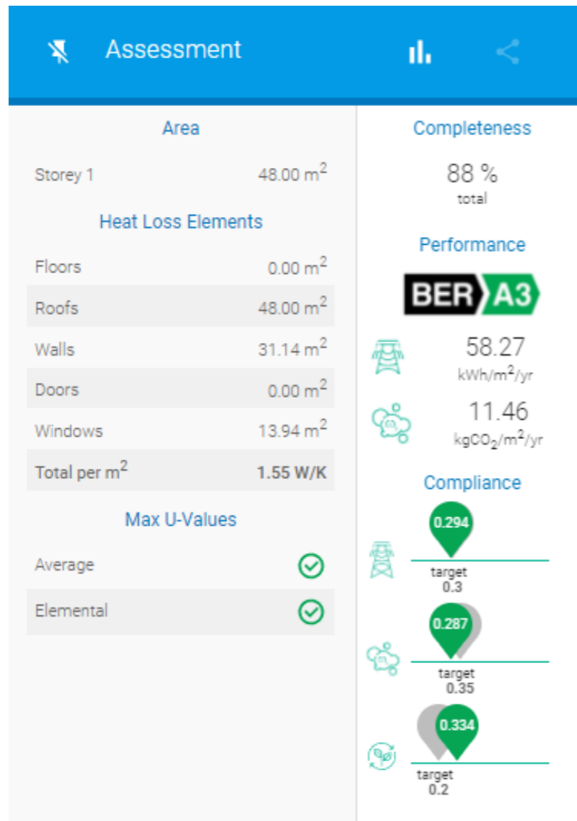
Figure 4.2.2: Part L Compliance – Primary Energy Breakdown
