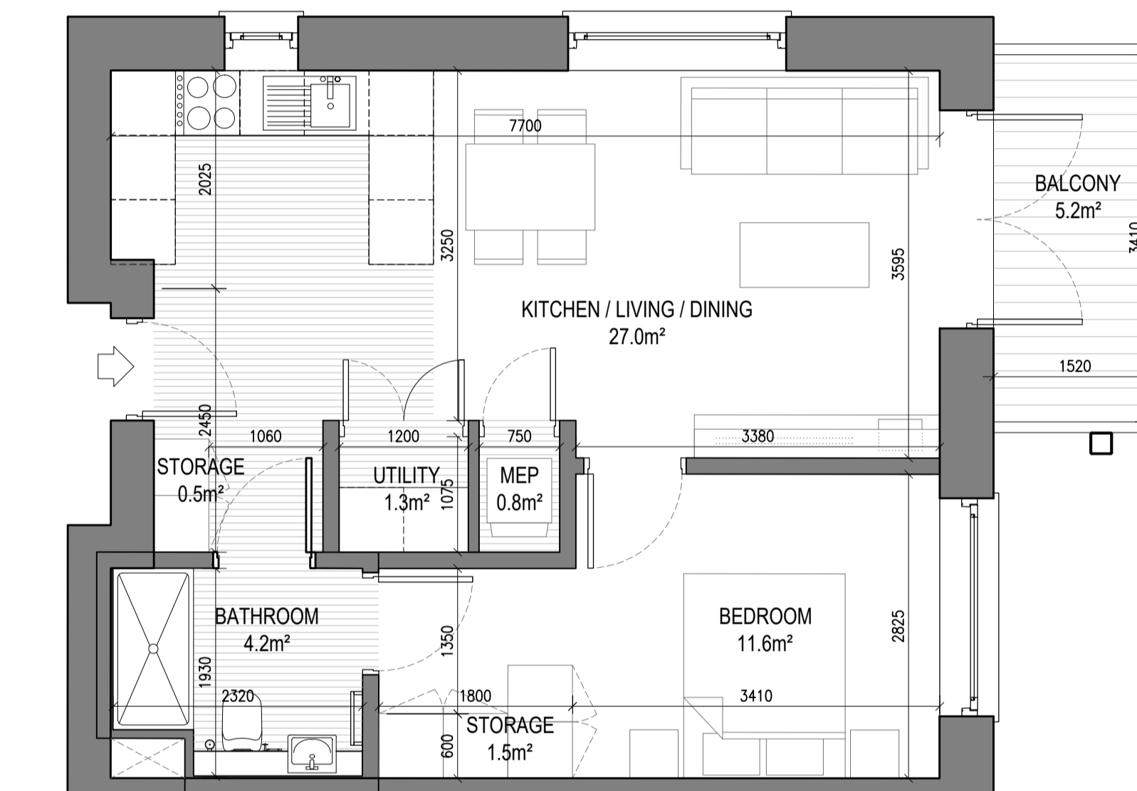
UNIT TYPE A1.4 1 Bed Unit - Floor Area: 49.40m 2 SCALE 1:50 REQUIRED (m 2 ) PROVIDED (m 2 ) STORAGE SPACE 3.0 3.3 PRIVATE AMENITY SPACE 5.0 5.2 AGGREGATE BEDROOM AREA 11.4 11.6 AGGREGATE KITCHEN / LIVING / DINING 23.0 27.0
