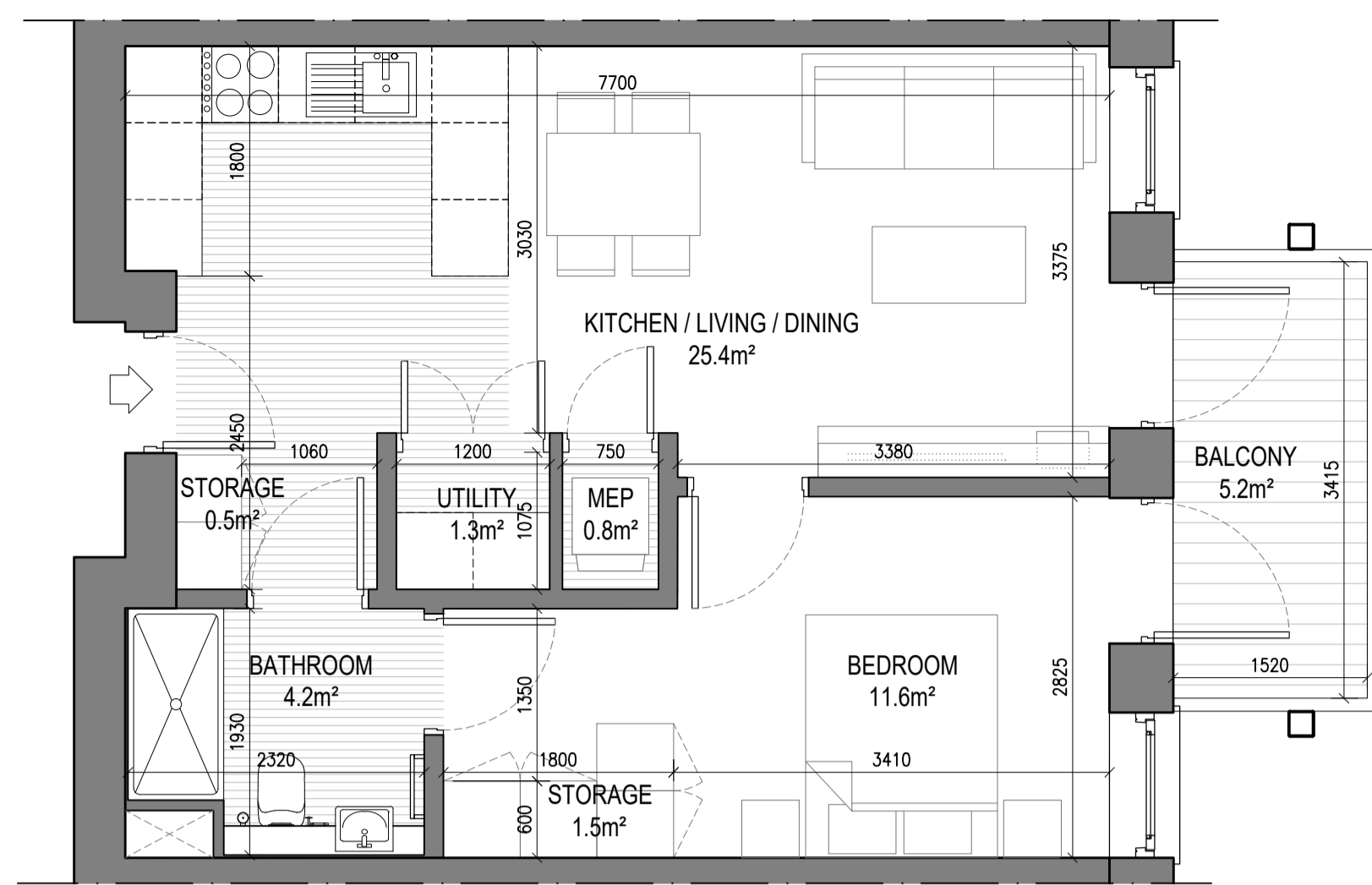
UNIT TYPE A1.1 1 Bed Unit - Floor Area: 47.84m 2 SCALE 1:50 REQUIRED (m 2 ) PROVIDED (m 2 ) STORAGE SPACE 3.0 3.3 PRIVATE AMENITY SPACE 5.0 5.2 AGGREGATE BEDROOM AREA 11.4 11.6 AGGREGATE KITCHEN / LIVING / DINING 23.0 25.4
