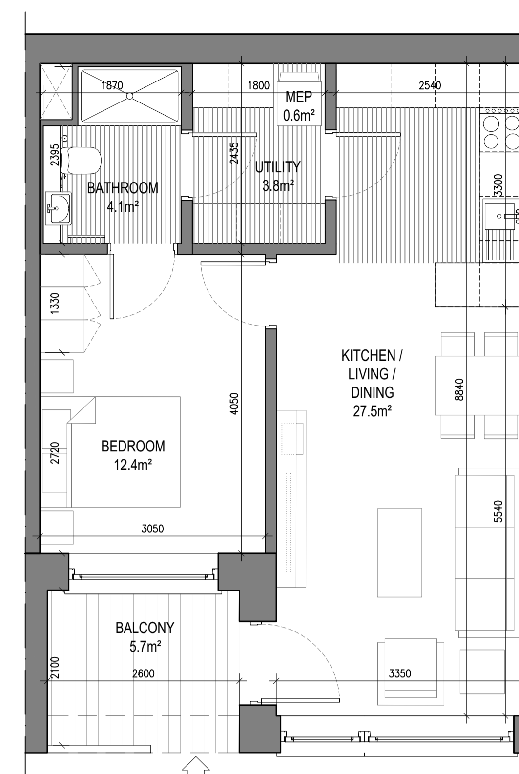
UNIT TYPE A2.4 1 Bed Unit - Floor Area: 50.86m 2 SCALE 1:50 REQUIRED (m 2 ) PROVIDED (m 2 ) STORAGE SPACE 3.0 3.8 PRIVATE AMENITY SPACE 5.0 5.7 AGGREGATE BEDROOM AREA 11.4 12.4 AGGREGATE KITCHEN / LIVING / DINING 23.0 27.5
