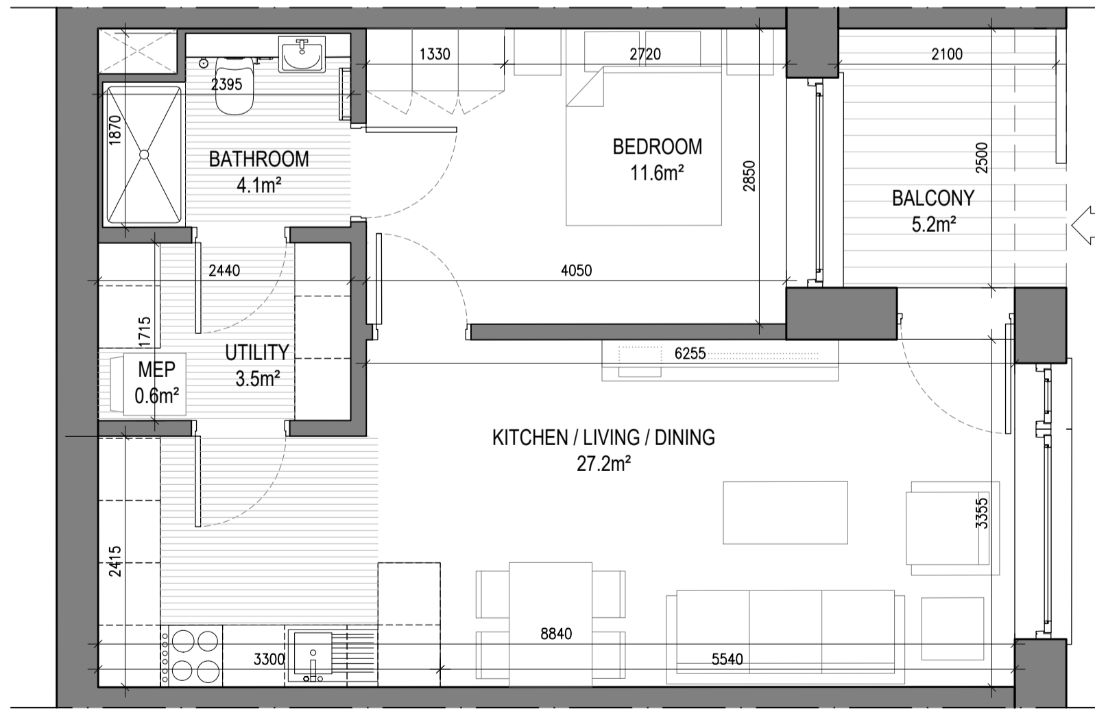
UNIT TYPE A2.2 1 Bed Unit - Floor Area: 49.55m 2 SCALE 1:50 REQUIRED (m 2 ) PROVIDED (m 2 ) STORAGE SPACE 3.0 3.5 PRIVATE AMENITY SPACE 5.0 5.2 AGGREGATE BEDROOM AREA 11.4 11.6 AGGREGATE KITCHEN / LIVING / DINING 23.0 27.2
