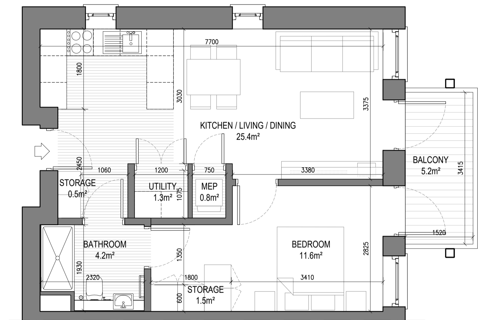
UNIT TYPE A1.2 1 Bed Unit - Floor Area: 47.84m 2 SCALE 1:50 REQUIRED (m 2 ) PROVIDED (m 2 ) STORAGE SPACE 3.0 3.3 PRIVATE AMENITY SPACE 5.0 5.2 AGGREGATE BEDROOM AREA 11.4 11.6 AGGREGATE KITCHEN / LIVING / DINING 23.0 25.4
