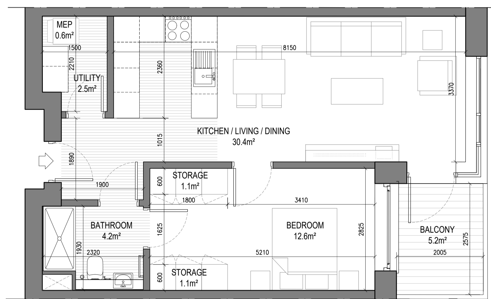
UNIT TYPE A2.1 1 Bed Unit - Floor Area: 54.80m 2 SCALE 1:50 REQUIRED (m 2 ) PROVIDED (m 2 ) STORAGE SPACE 3.0 4.7 PRIVATE AMENITY SPACE 5.0 5.2 AGGREGATE BEDROOM AREA 11.4 12.6 AGGREGATE KITCHEN / LIVING / DINING 23.0 30.4
